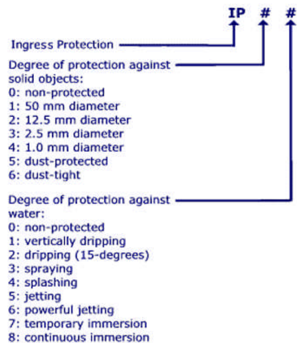
Figure 1—Ingress Protection (IP) code definitions
