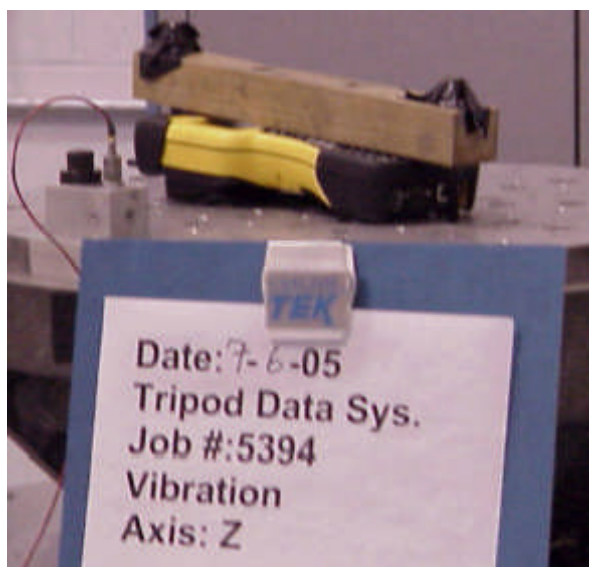
Figure 5—MIL-STD-810F Method 514.5, vibration test
